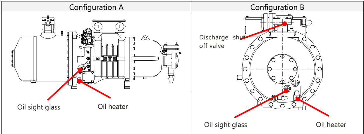
Fig. 13: positions of the oil heater and sight glass
