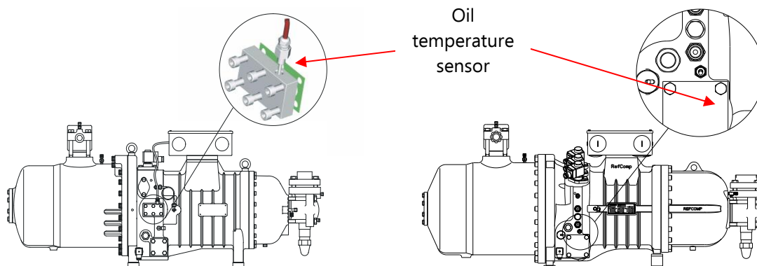
Fig. 42: position on compressor for oil temperature monitoring sensor
