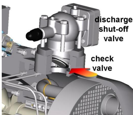
Fig. 31: check valve
