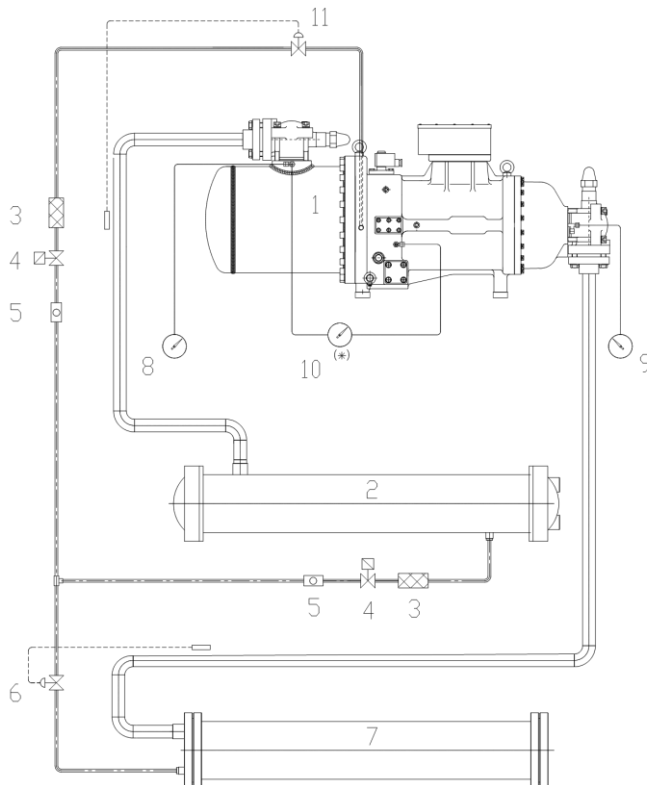
Fig. 53: injection of refrigerant (saturated liquid) via thermostatic expansion valve; To inject the refrigerant into the compressor, an expansion device must be installed; this may be:
