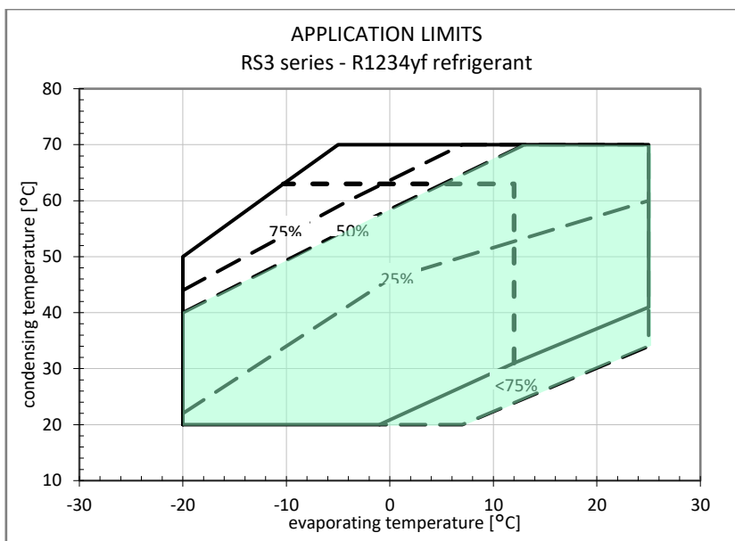
Fig. 28 Example of limited application limit at 50% load
