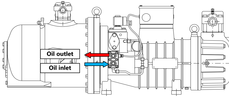
Fig. 58: Models RS3-H040÷060/L030÷050
