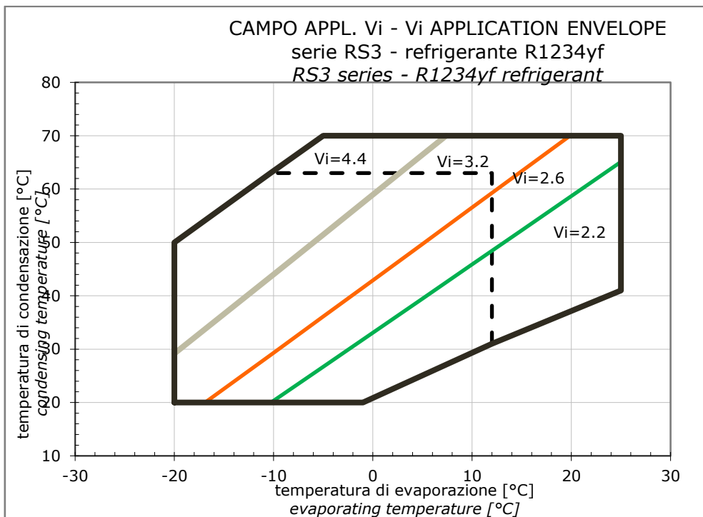
Fig. 8: V_i values recommended with R1234yf
