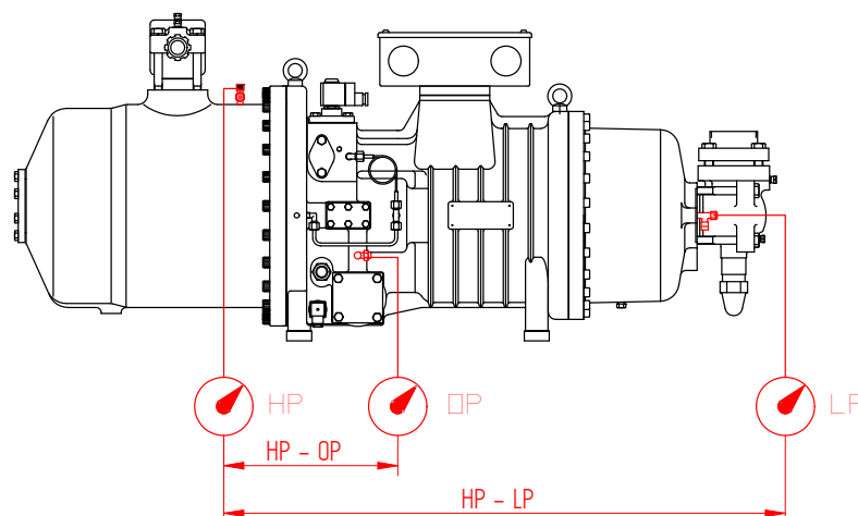
Fig. 15: measuring the HP, OP and LP pressure values in the RS3 series
