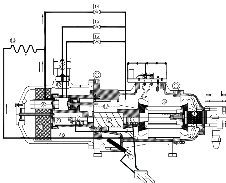
Fig. 21: capacity control at 100% step
