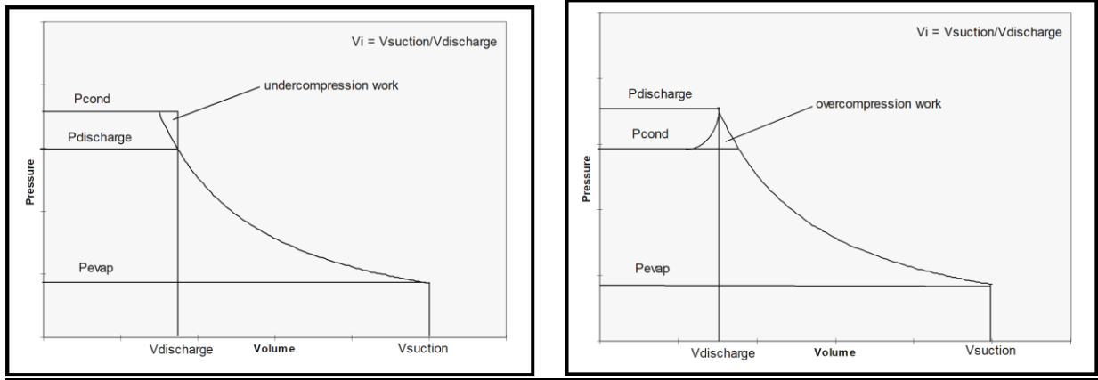
Fig. 7: the compression process on the p-V diagram;
