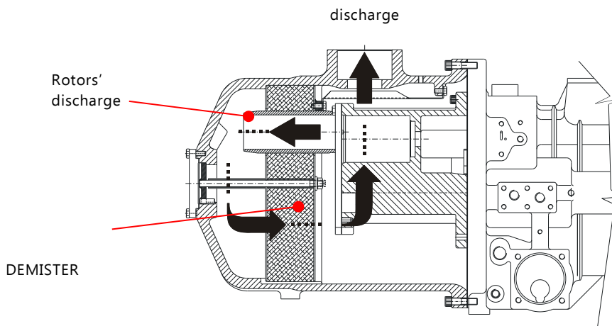
Fig. 10: specific position of the oil separator both for the RS3 series;
