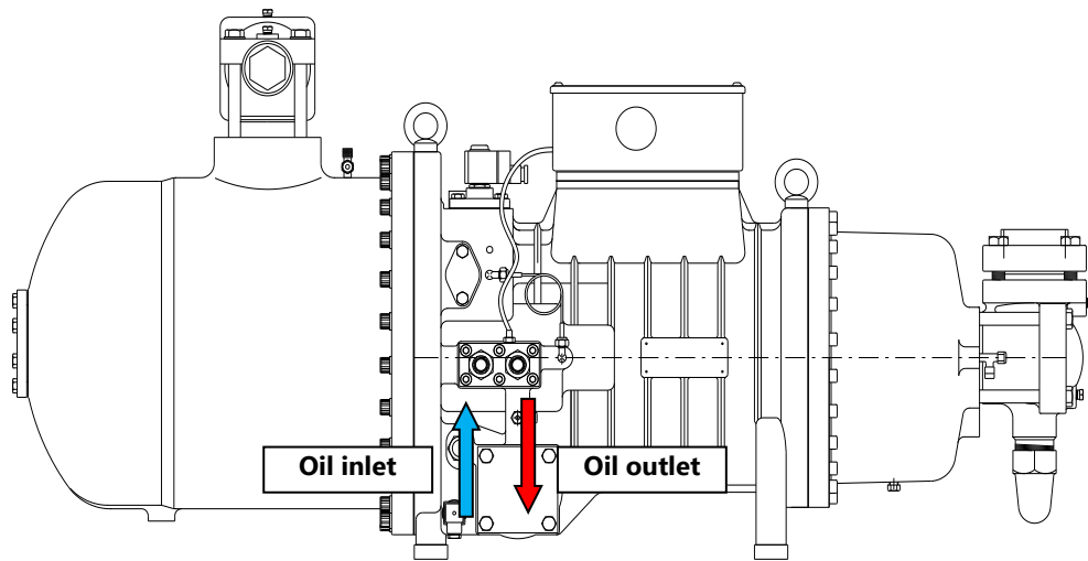
Fig. 60: Models RS3-H140÷240/L110÷200
