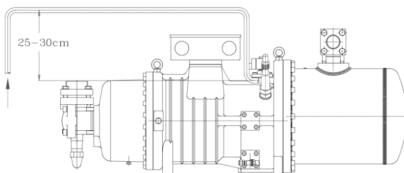
Fig. 54: layout of the liquid injection line;
