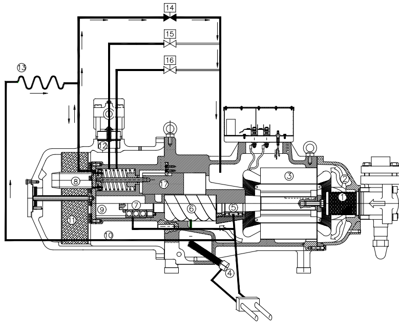
Fig. 18: Minimum capacity control oil circuit
