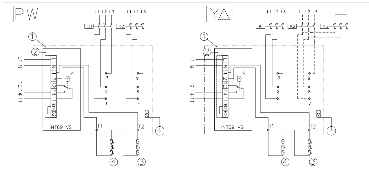
Fig. 40: electrical connections to the INT 69 B2 module (part-winding and star delta);
