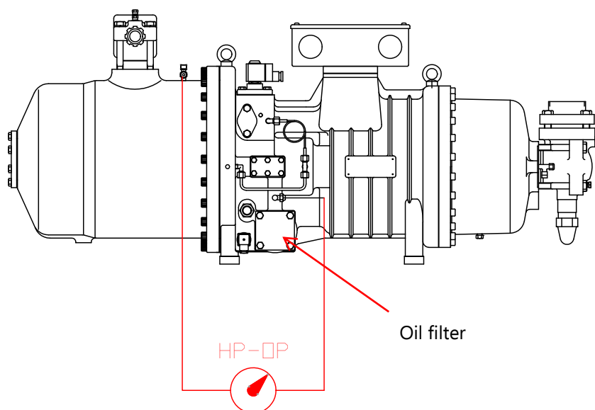
Fig. 12: position of the oil filter in the RS3 series compressors (in models H040÷060/L030÷050 the filter is located inside the oil separator) and definition of the HP-OP pressure drop across the filter
