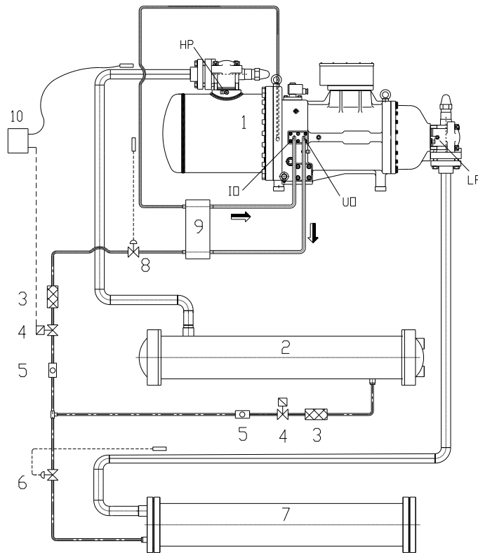
Fig. 56: oil cooling with oil/refrigerant fluid heat exchanger
