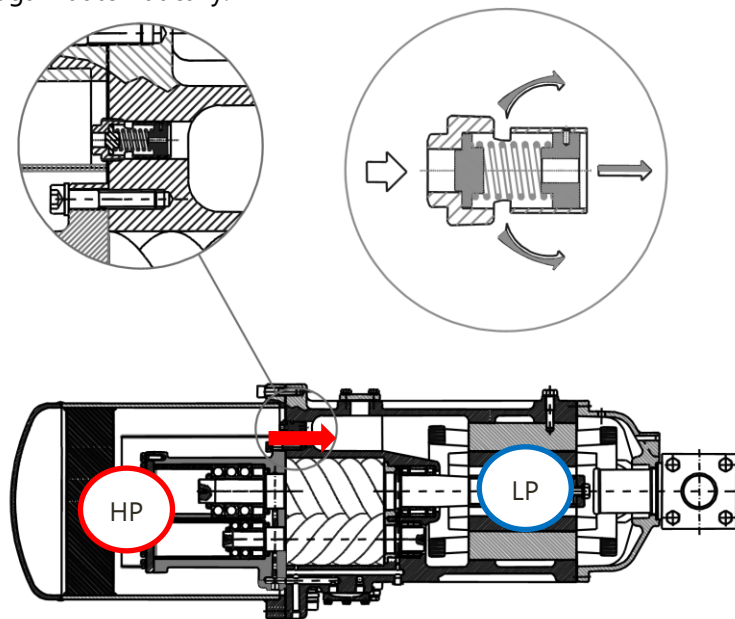
Fig. 30: safety valve shape and position
