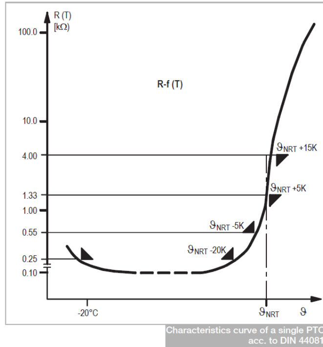
Fig. 43 Characteristics response curve of a single PTC
