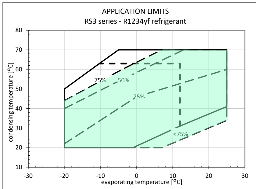
Fig. 27 Example of limited application limit at 75% load
