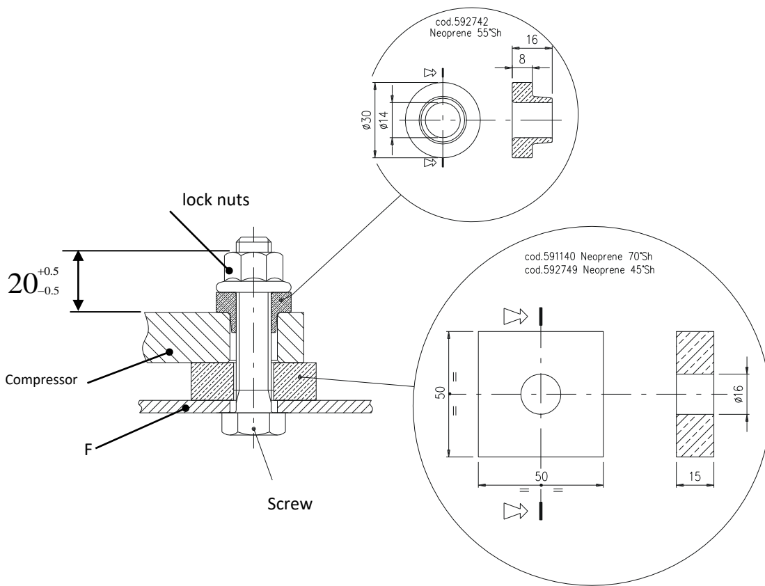
Fig. 34: assembly diagram for the rubber vibration dampers;
