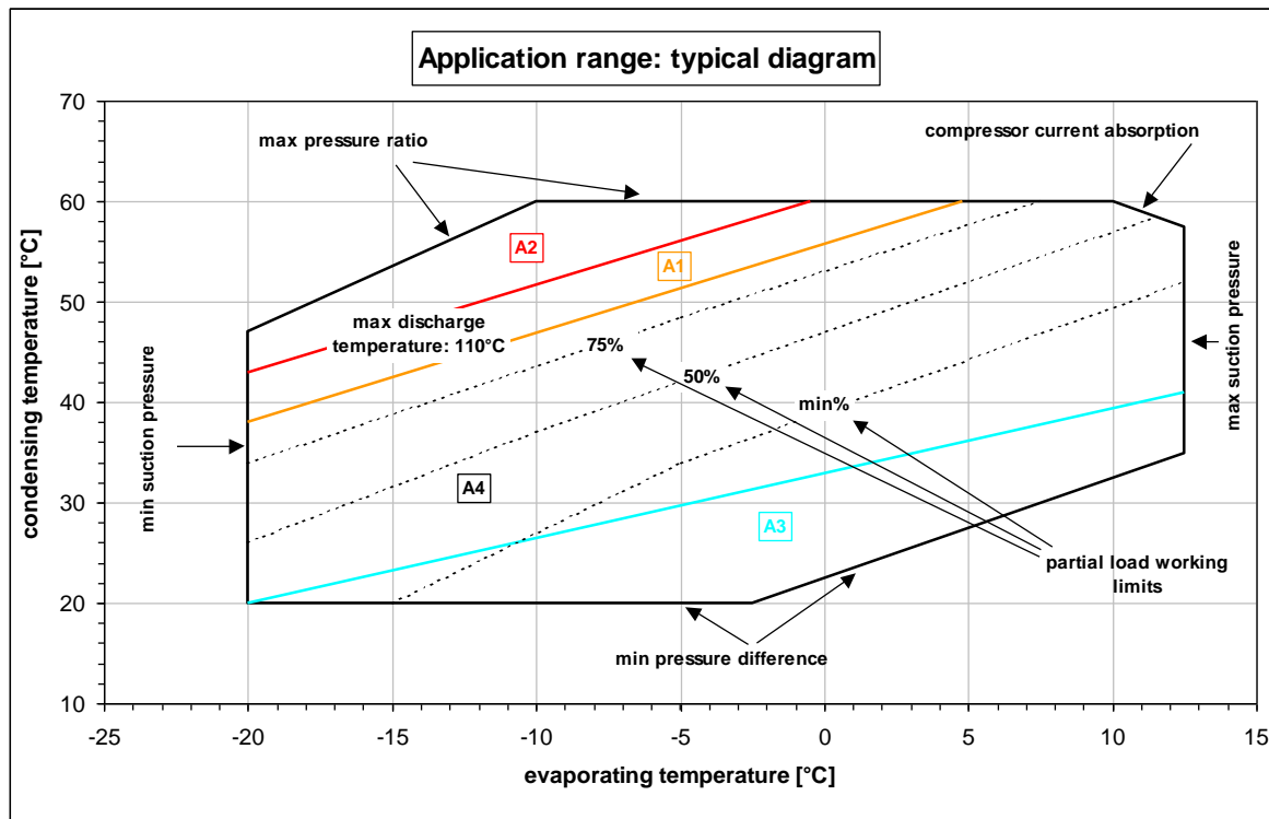
Fig. 52: typical application range;
