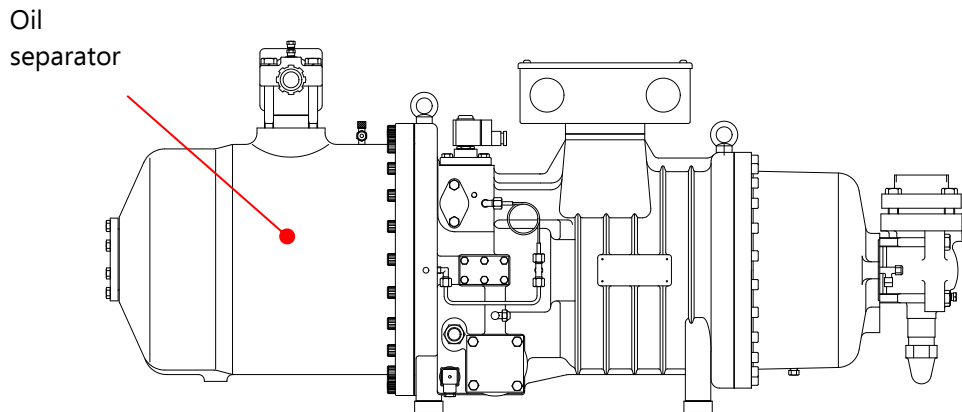
Fig. 10: specific position of the oil separator both for the RS3 series;
