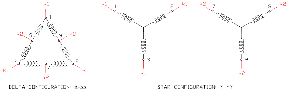
Fig. 37: internal winding connections for the motors with part-winding configuration
