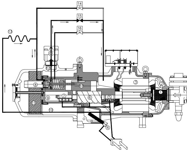
Fig. 19: capacity control at 50% step
