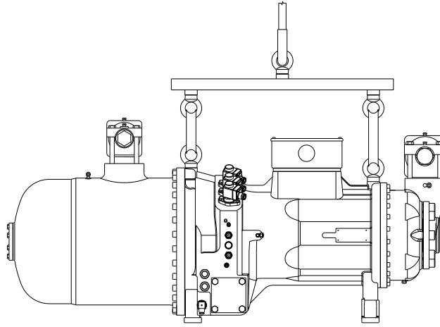
Fig. 51: anchor points for lifting the compressor;
