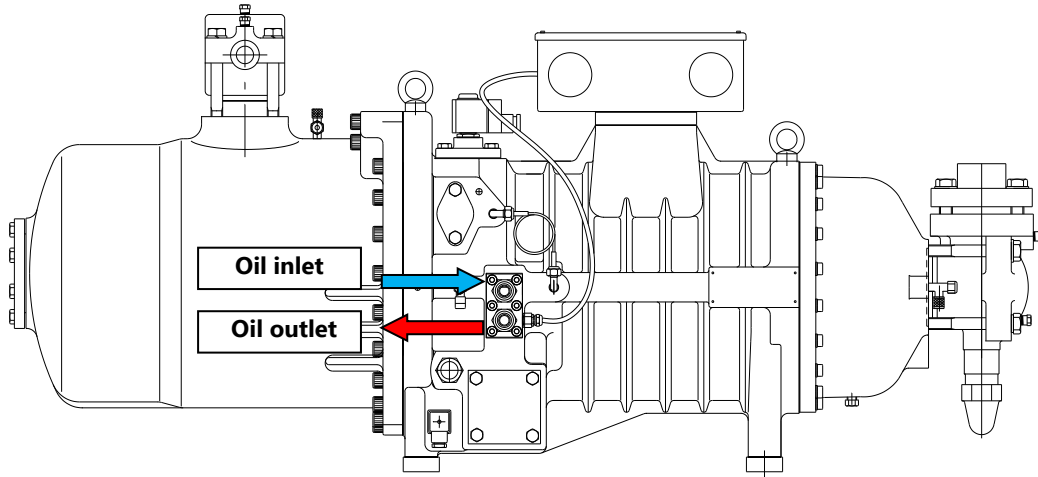
Fig. 59: Models RS3-H070/080
