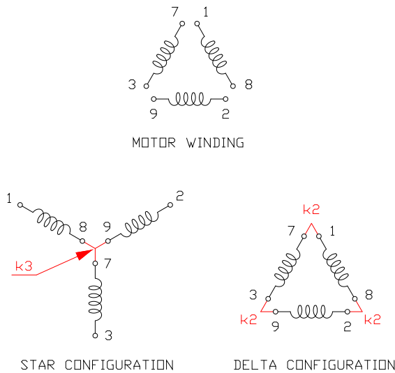
Fig. 38: internal winding connections for the motors with star-delta configuration
