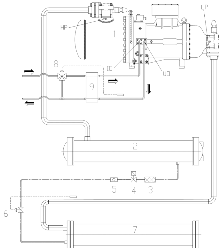
Fig. 55: oil cooling with oil/water heat exchanger
