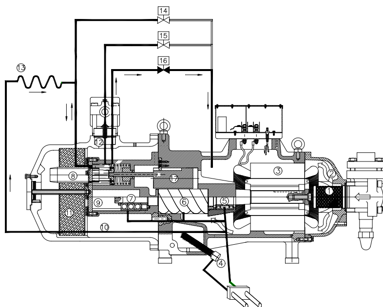
Fig. 20: capacity control at 75% step;
