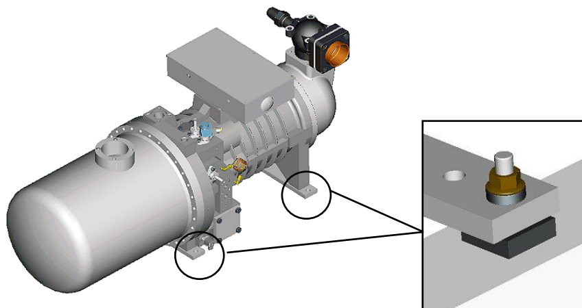
Fig. 32: position of the rubber vibration damper underneath the 4 feet of the compressors;
