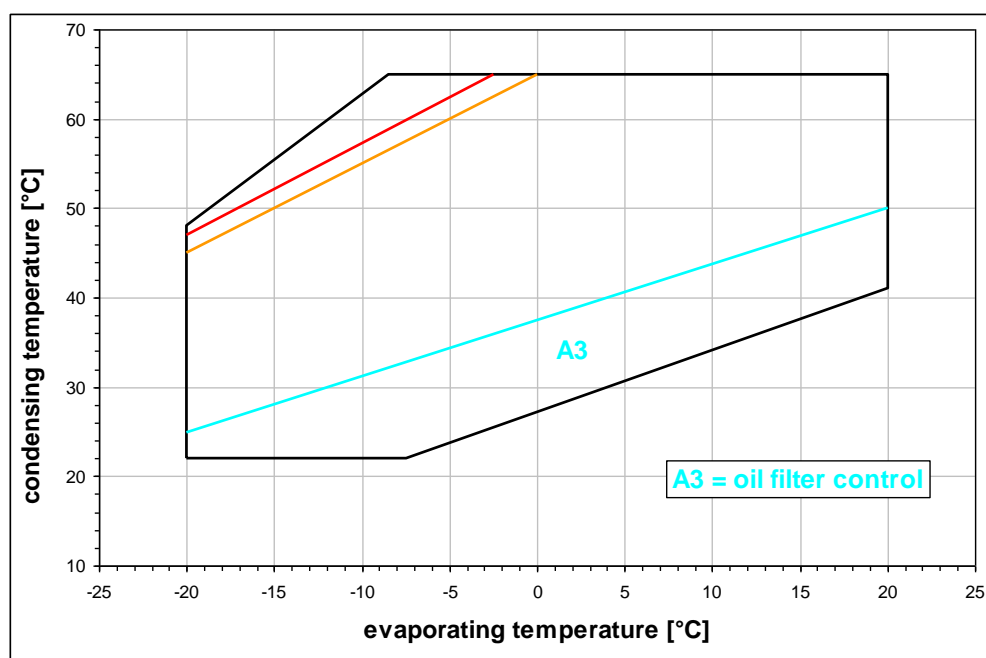
Fig. 16: generic application limit for series RS3 compressors
