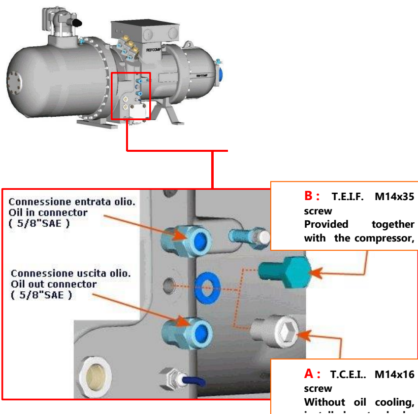
Fig. 57: oil inlet/outlet connection location for the external oil cooling circuit;
