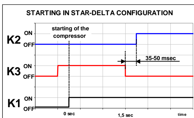
Fig. 39: connection diagrams to the three-phase network and time charts for the activation of contactors K1, K2 and K3 in the two compressor starting modes: star-delta and part-winding;
