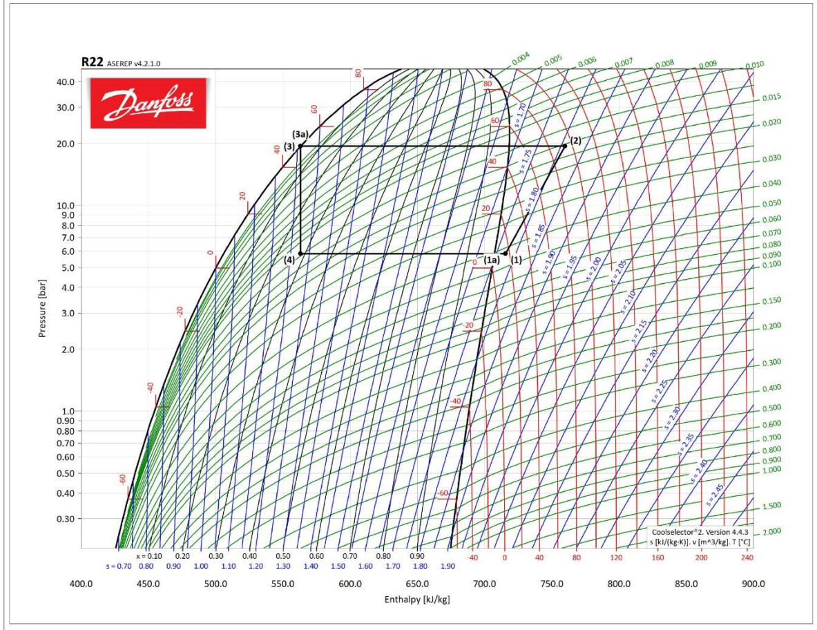
Detailed log(p)-h diagram
