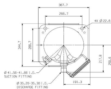
(VIEW W/O TERMINAL BOX)
