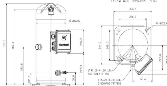
(VIEW W/O TERMINAL BOX)
